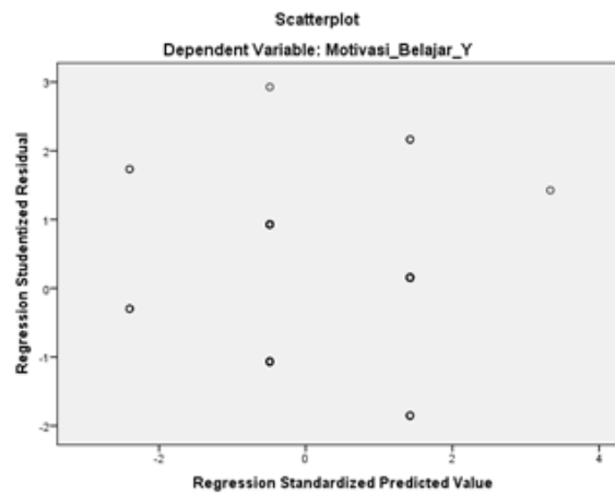
Figure 2 : Scatterplot of Heteroscedasticity Test (Model 2)
