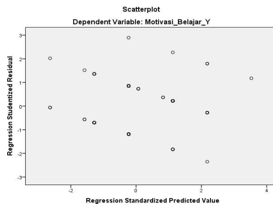
Figure 3 : Scatterplot of Heteroscedasticity Test (Model 3) (Source: Processed Data Results Using SPSS, 2020)
