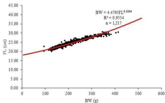
Figure 6. LWR of BLT from Indian Ocean, WNT
