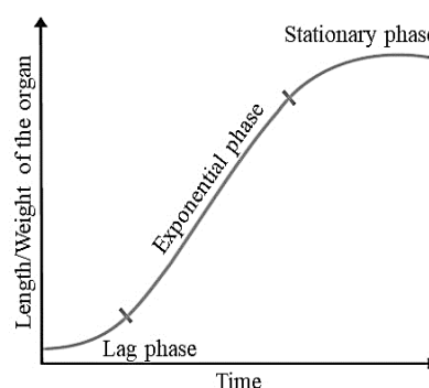
Figure 2. Sigmoid curve (S curve)
