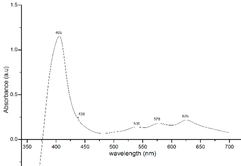
Figure 1. The absorption spectrum of chlorophyll Alfalfa ( Medicago sativa L. )
