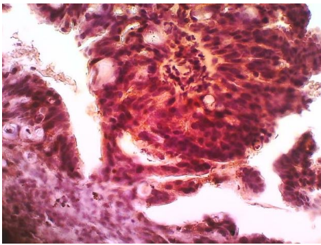
Figure 6. High ERCC1 expression
