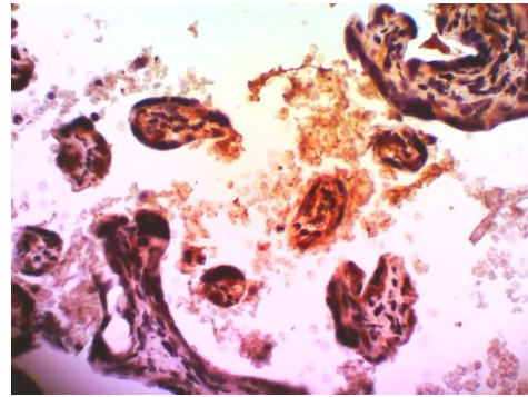
Figure 1. Positive control of CTR1
